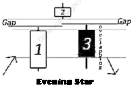
Gambar 2.20 Evening Star
