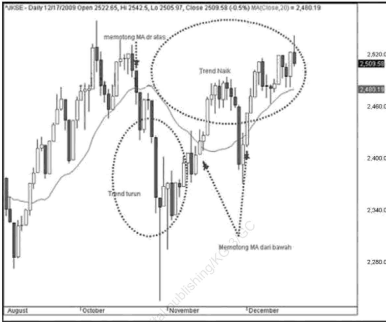
Gambar 6.1 SMA Trend
