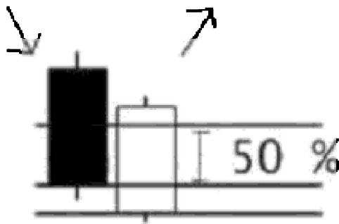
Gambar 2.15 Piercing Pattern
