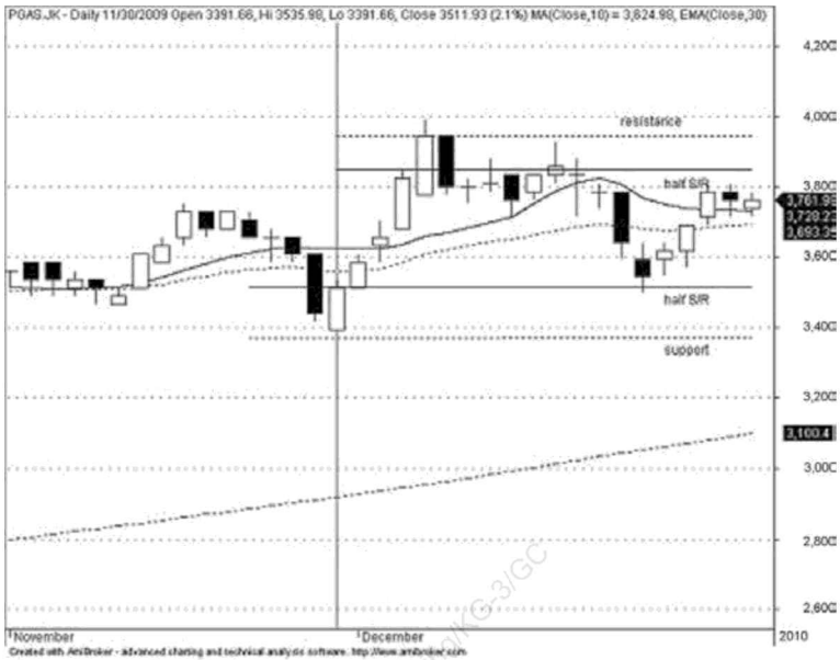
Gambar 7.5 Half S/R
