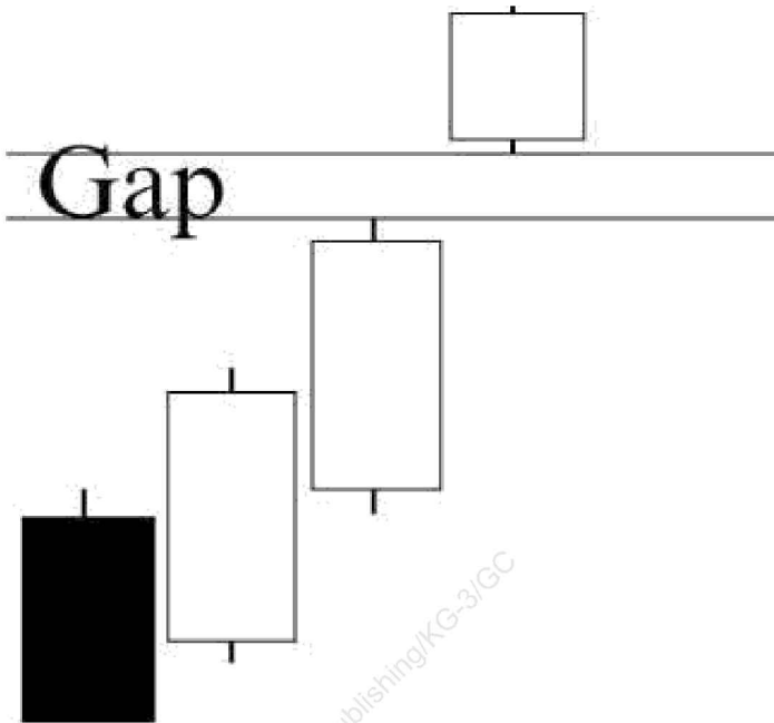
Gambar 3.7 Gap Sample
