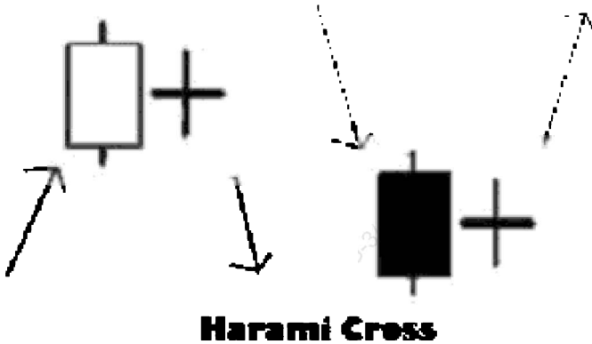
Gambar 2.17 Harami Cross
