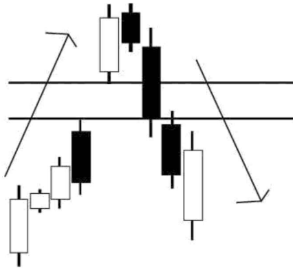
Gambar 3.9 Closing Gap
