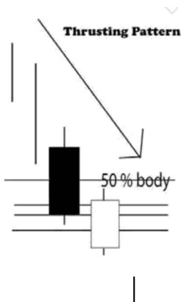
Gambar 2.27 Thrusting Pattern
