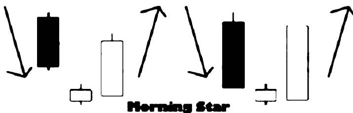
Gambar 2.19 Morning Star
