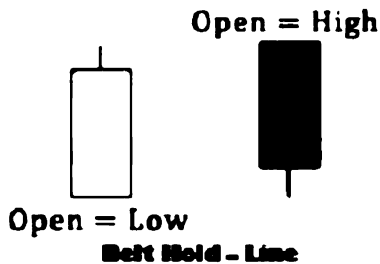
Gambar 2.7 Belt Hold-Line
